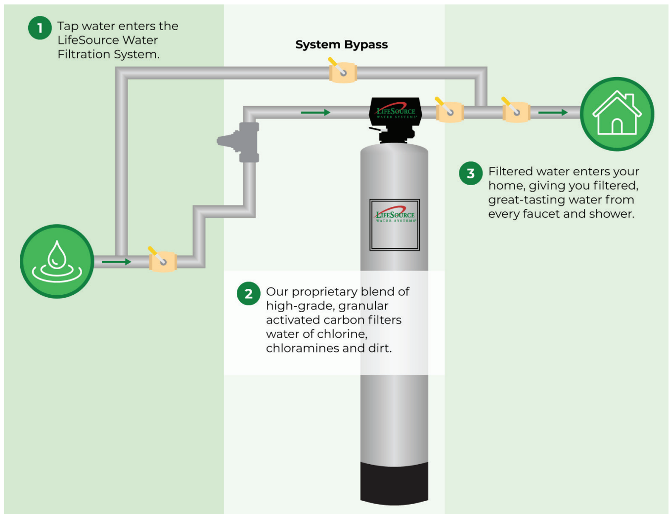
Figure 6 - Estate Filter Water Loop Example
