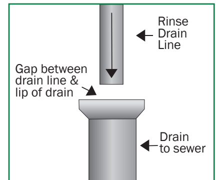
Figure 4 - Air Gap Illustration
