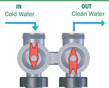
Figure 11: ScaleSolver Valve In SERVICE Position
