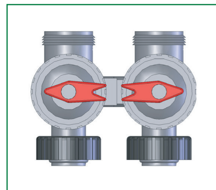
Figure 3 - ScaleSolver Valve IN Bypass Position
