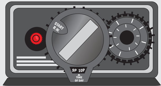
Figure 6 - Control knob in BACKWASH position.
