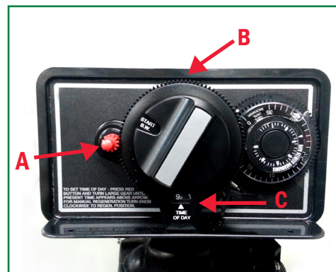
Figure 9 - Resetting self-rinse timer.
